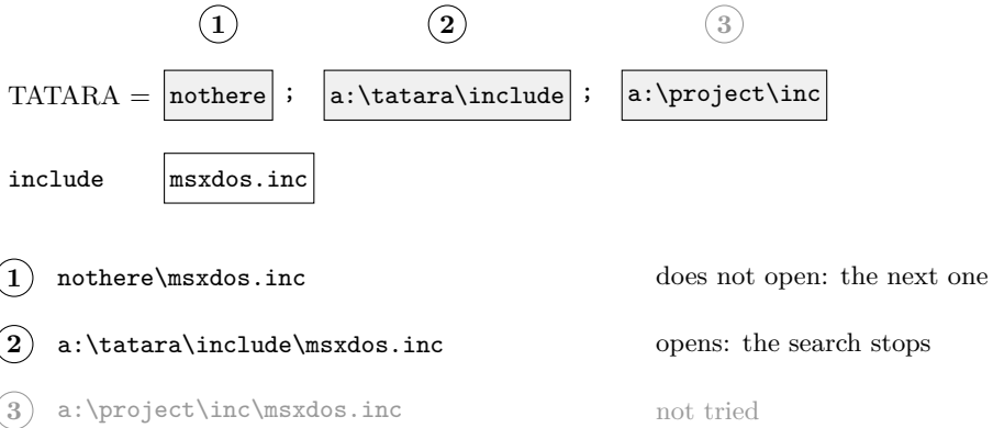
Figure I.1: How the value of TATARA and the name in an INCLUDE line become the names that are tried, in order.
