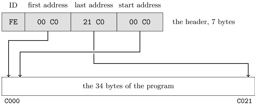
Figure 26.1: The BLOAD header of HELLO B .BIN, and the three addresses it holds.
