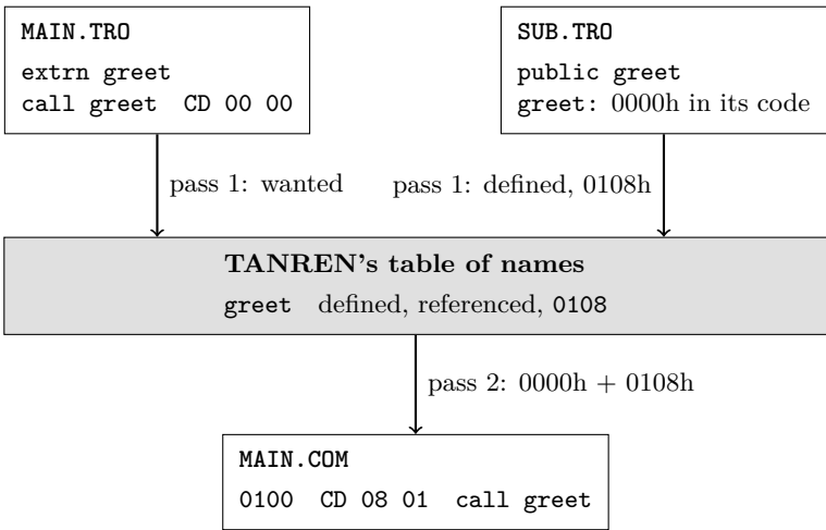
Figure 25.1: How greet , external in MAIN and public in SUB , gets its value.
