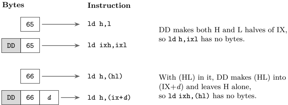
Figure 9.1: One prefix for the whole instruction: what DD does to two instructions.
