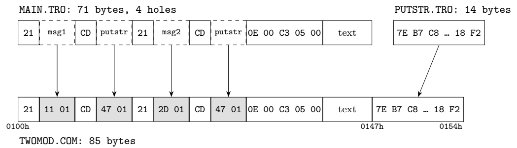
Figure 2.2: Linking MAIN.TRO and PUTSTR.TRO into TWOMOD.COM.
