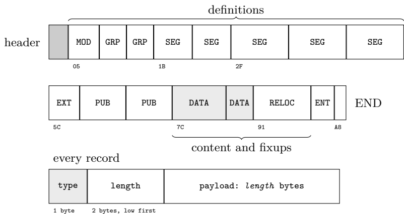
Figure F.1: OBJ.TR0 as a row of records, and the layout of one record. The width of each box is its size in bytes.
