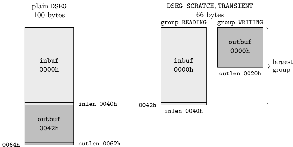
Figure 10.1: The same four variables in a plain data segment and in a transient one, drawn to scale.
