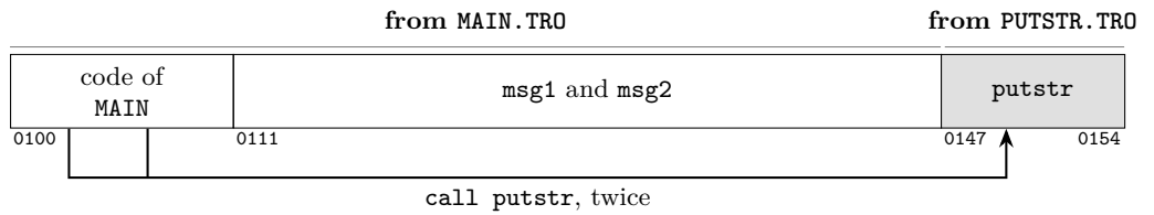
Figure 28.2: TWOMOD.COM in memory. Both calls in MAIN go to putstr , at 0147h.
