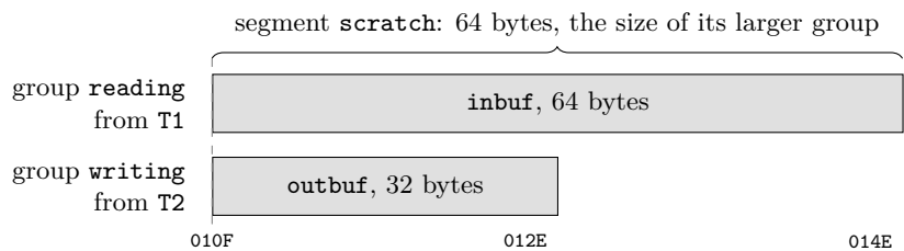
Figure 24.2: Two groups of the transient segment scratch, from two modules, at the same address.
