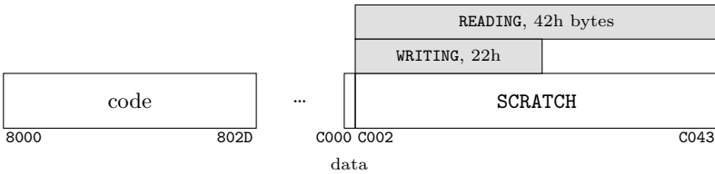
Figure 29.1: LAYOUT linked at 0100h, and with the code at 8000h and the data at C000h. In both, the two groups of SCRATCH start at the same address.
