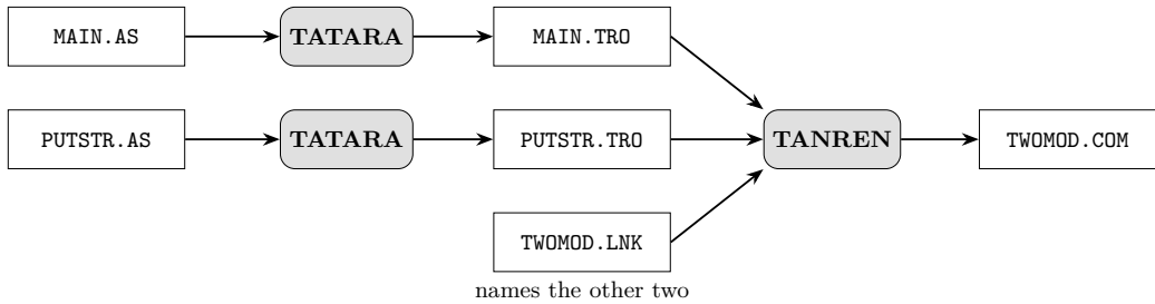
Figure 28.1: How BUILD.BAT makes TWOMOD.COM.
