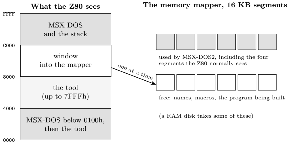
Figure G.1: The Z80’s 64 KB while TATARA or TANREN runs, and the mapper segments behind the window.
