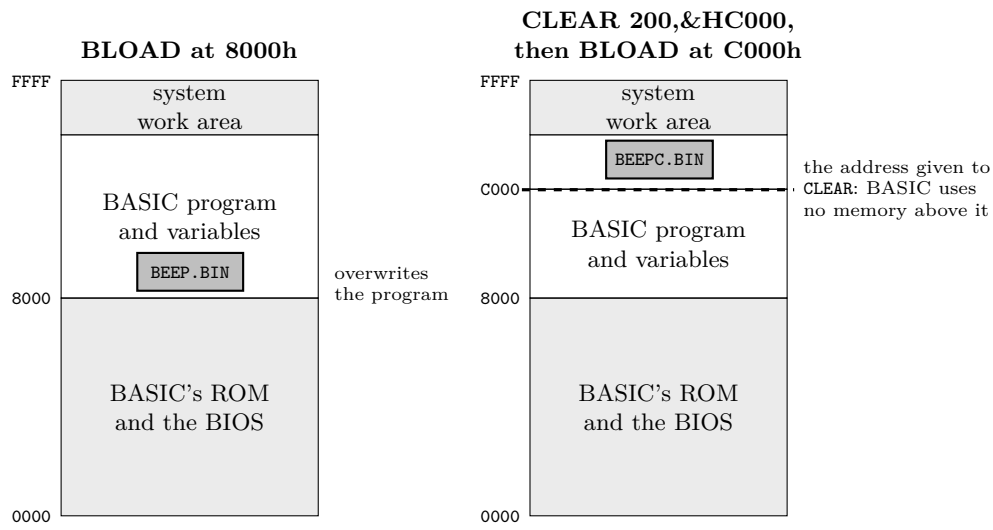
Figure 32.1: MSX-BASIC's memory, with the file at 8000h and at C000h.
