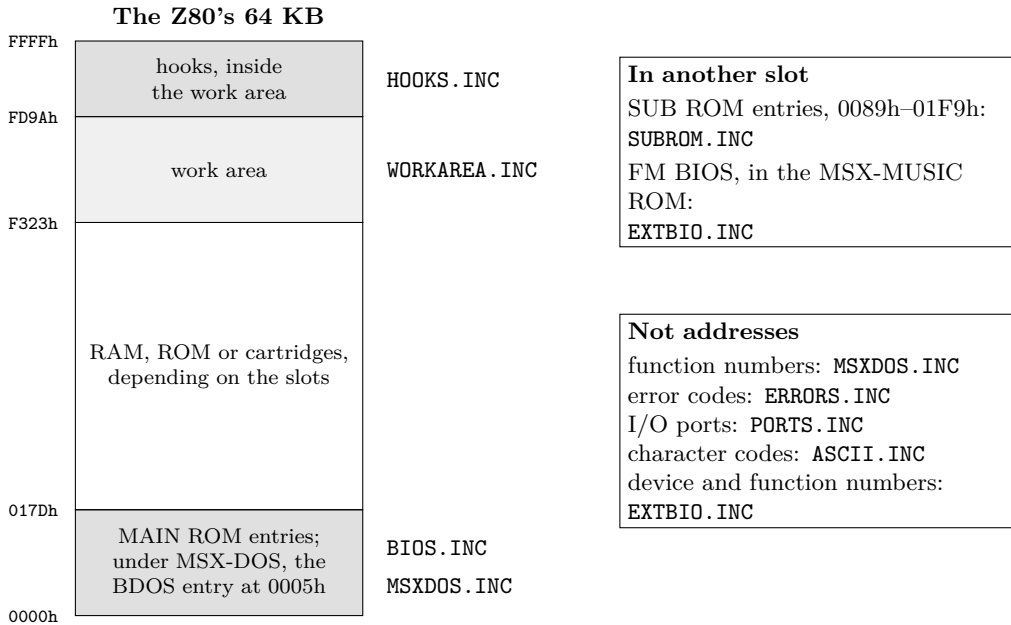
Figure K.1: Where the addresses named by the include files are.
