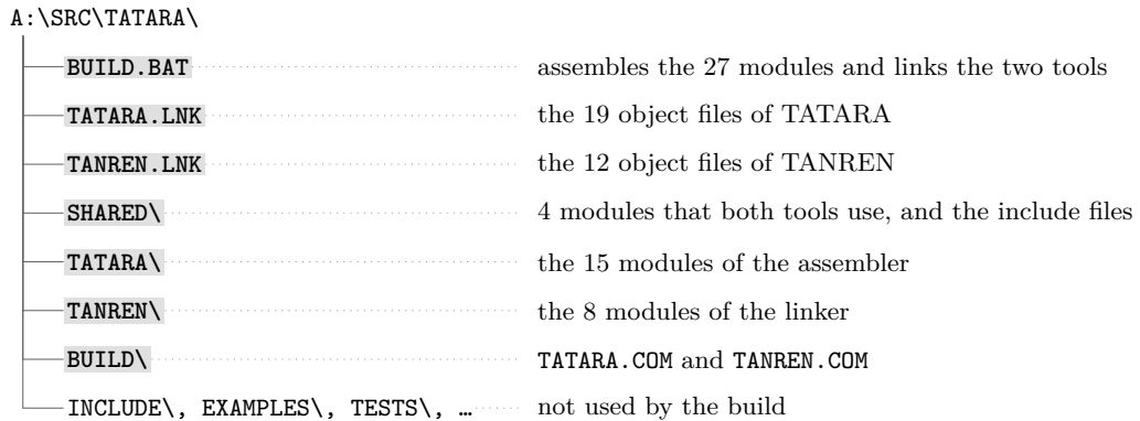
Figure 35.1: The source tree, and what the build uses from it.
