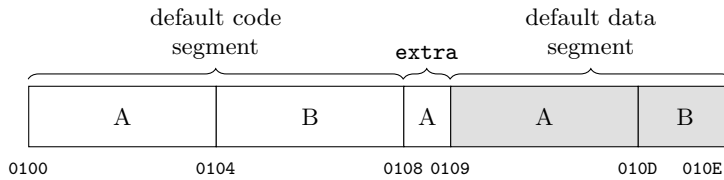
Figure 24.1: The memory of tanren a b . Each box is one module's part of a segment; the shaded ones are data.
