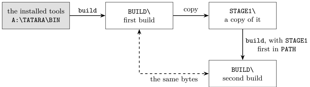
Figure 35.3: Building the tools twice: the second time with the tools that the first build made.
